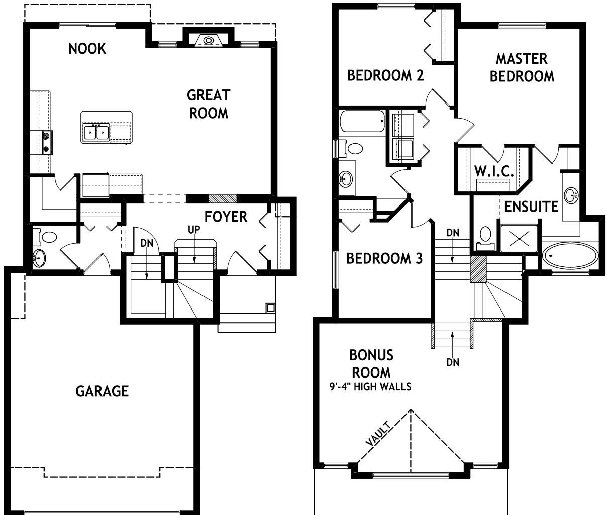
THE SEVILLE 1786 SQUARE FEET
